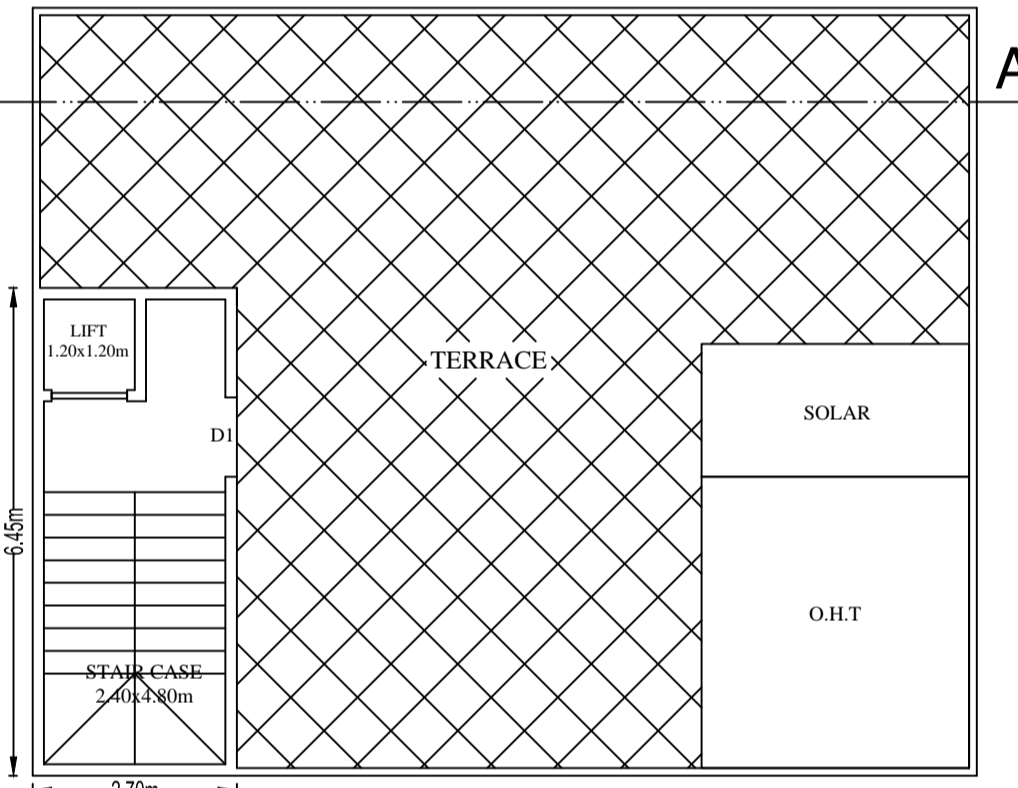
PROPOSED TERRACE FLOOR PLAN
