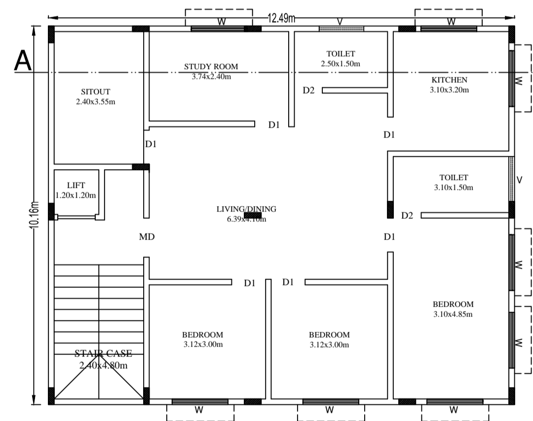
PROPOSED TYPICAL FIRST & SECOND FLOOR PLAN
